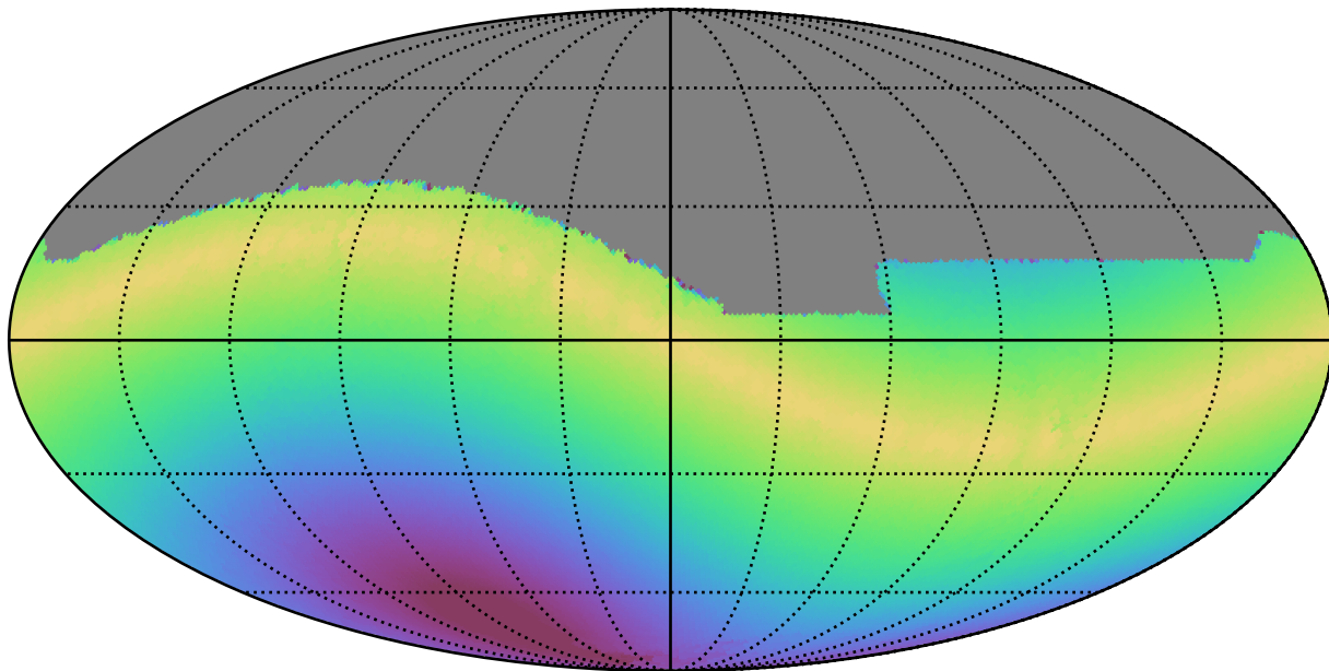
ddf_acor_sf20_lsf30_lsr10_v3.4_10yrs All sky i band: Max solarElong
