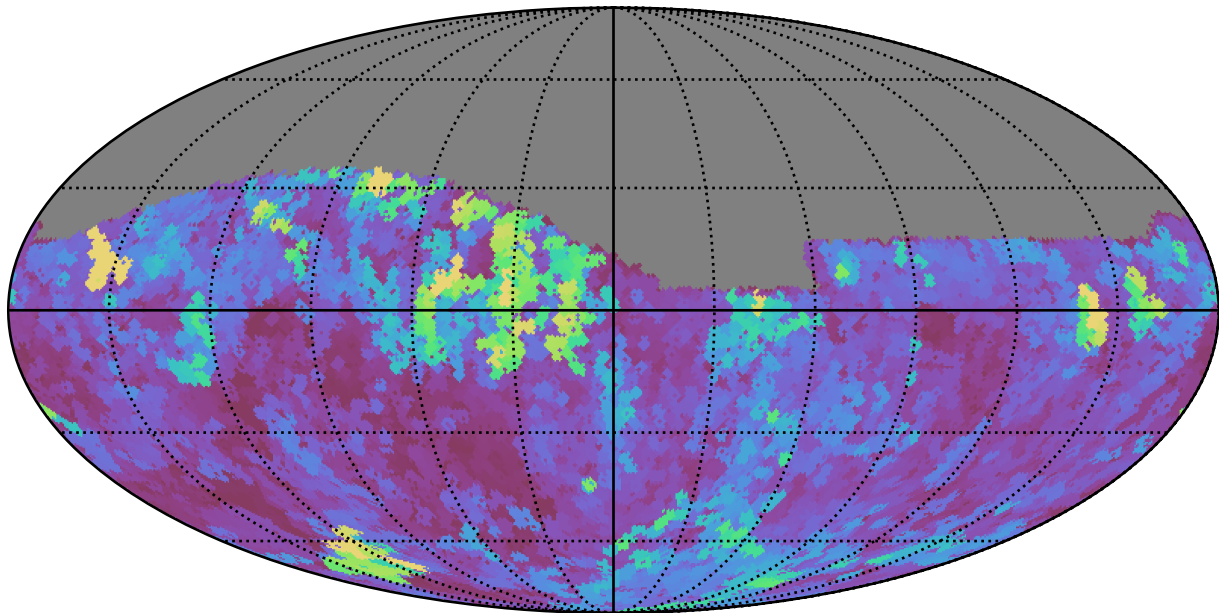
ddf_acor_sf20_lsf30_lsr10_v3.4_10yrs Yr 1 i band: Max seeingEff
