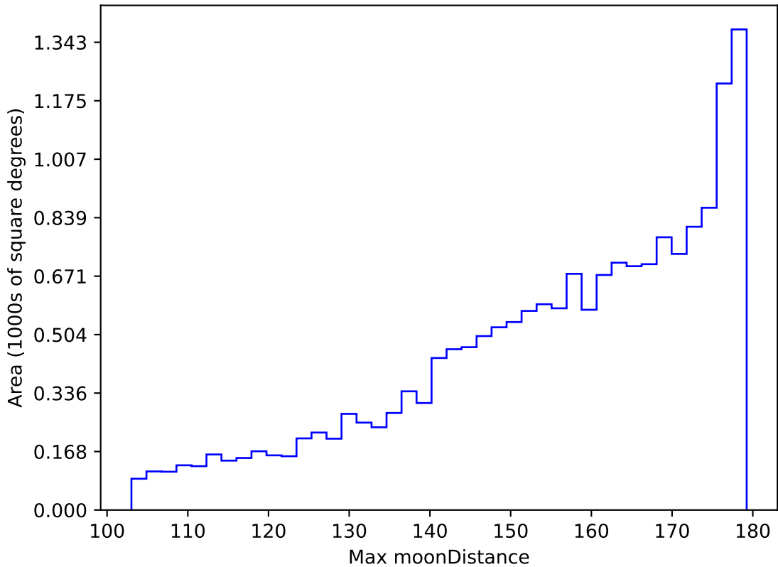
ddf_acor_sf20_lsf30_lsr10_v3.4_10yrs WFD i band: Max moonDistance
