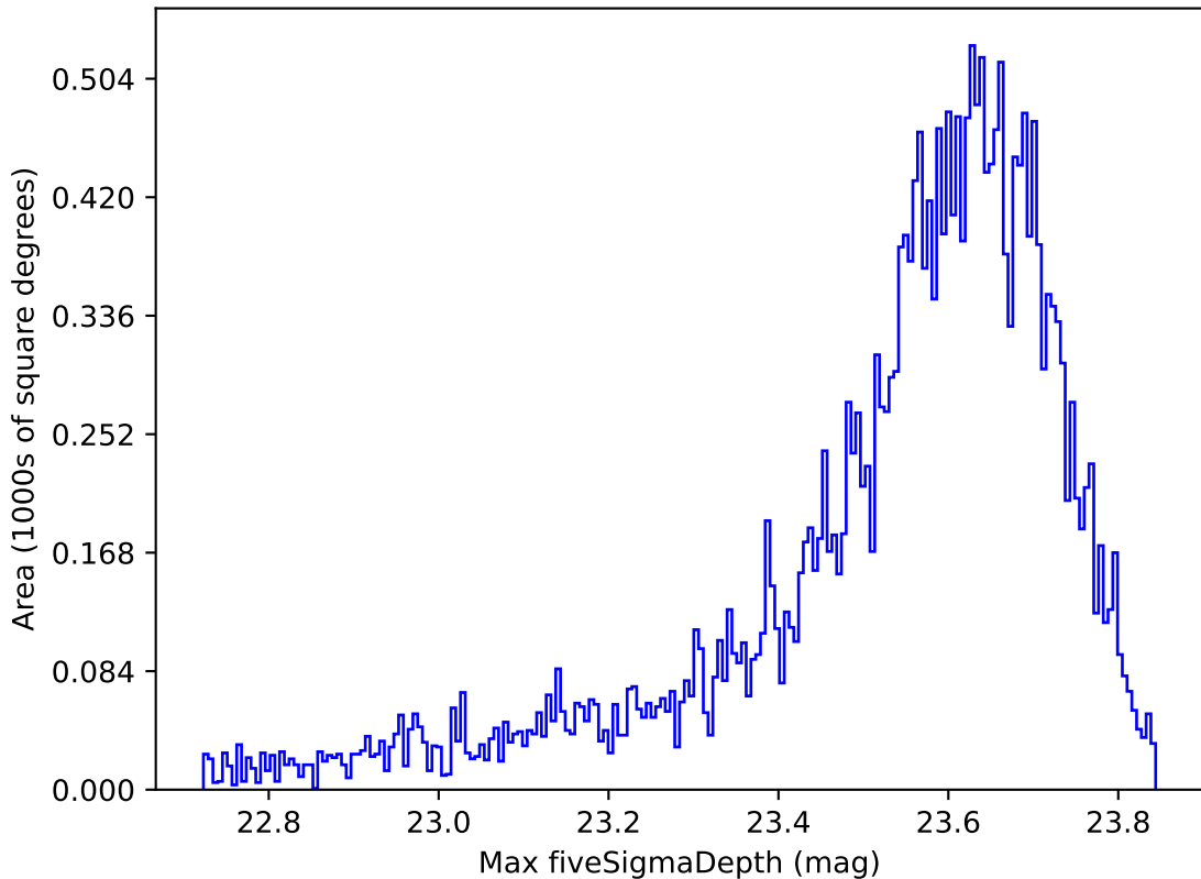
ddf_acor_sf20_lsf30_lsr10_v3.4_10yrs All sky z band: Max fiveSigmaDepth
