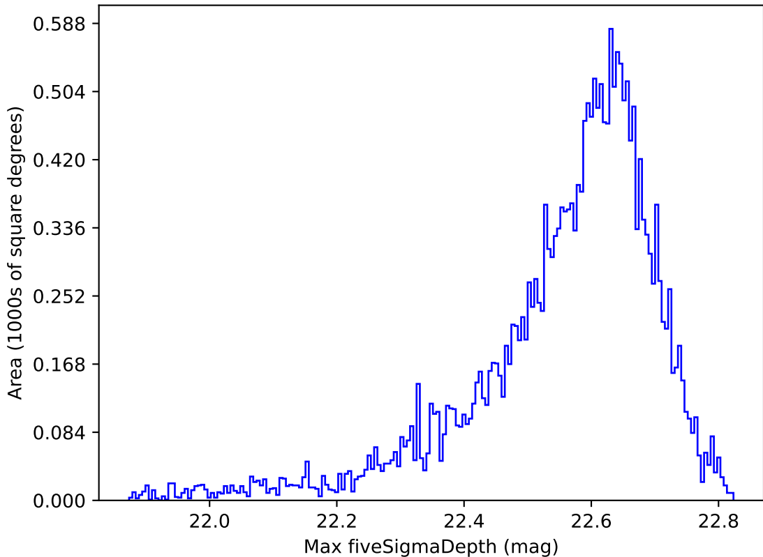
ddf_acor_sf20_lsf30_lsr10_v3.4_10yrs All sky y band: Max fiveSigmaDepth
