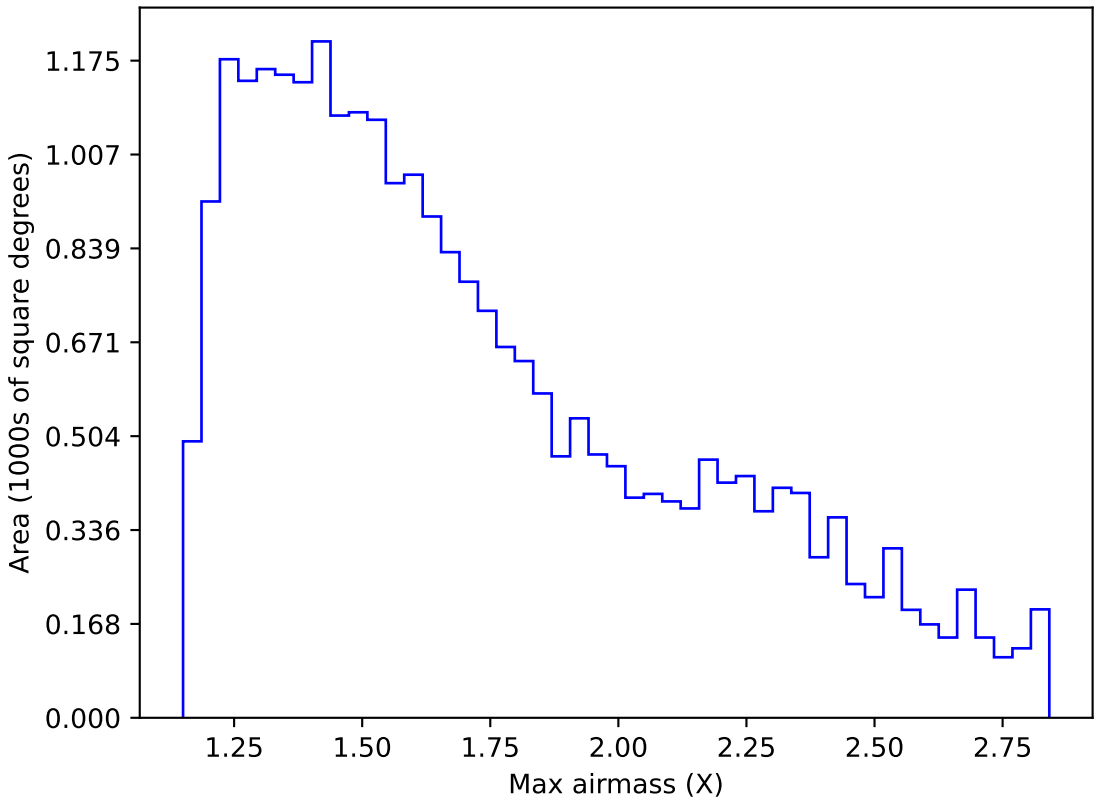
ddf_acor_sf20_lsf30_lsr10_v3.4_10yrs Yr 1 i band: Max airmass
