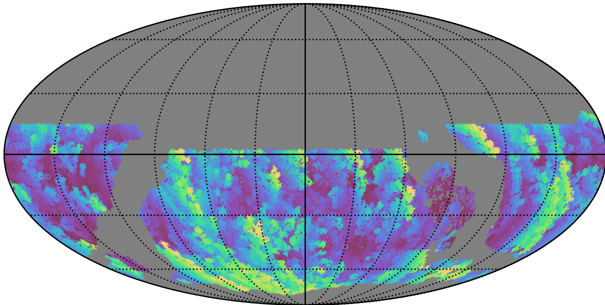
ddf_acor_sf20_lsf30_lsr10_v3.4_10yrs WFD u band: Max airmass
