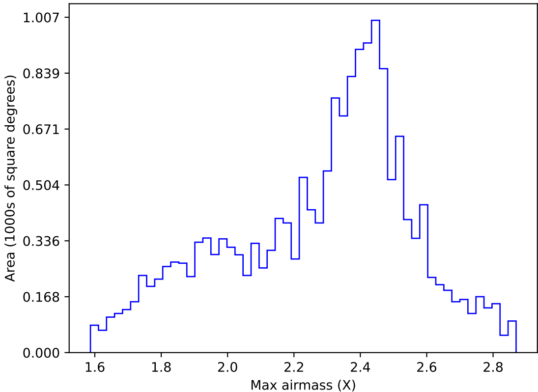
ddf_acor_sf20_lsf30_lsr10_v3.4_10yrs WFD r band: Max airmass
