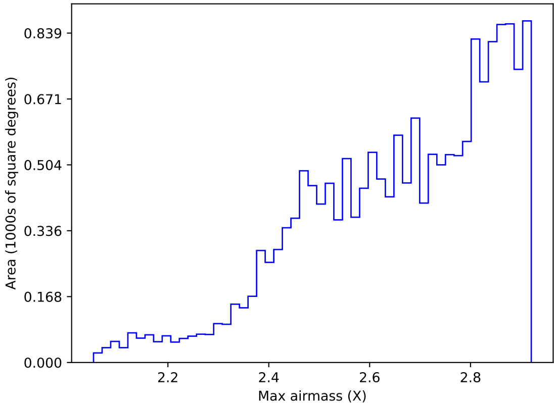
ddf_acor_sf20_lsf30_lsr10_v3.4_10yrs WFD all bands: Max airmass
