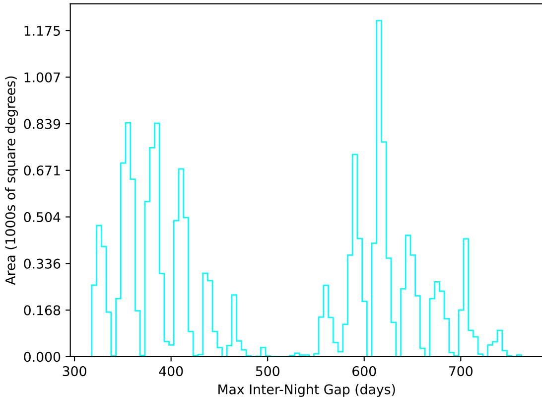
ddf_acor_sf20_lsf30_lsr10_v3.4_10yrs WFD u band: Max Inter-Night Gap
