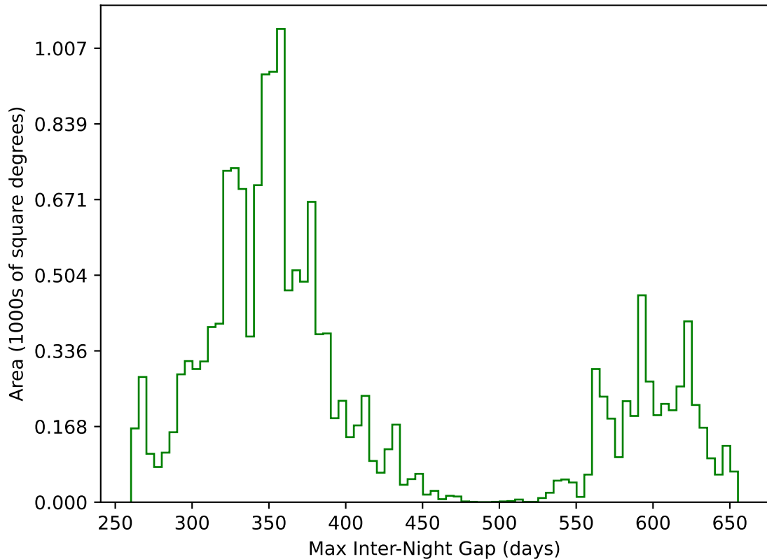
ddf_acor_sf20_lsf30_lsr10_v3.4_10yrs WFD g band: Max Inter-Night Gap
