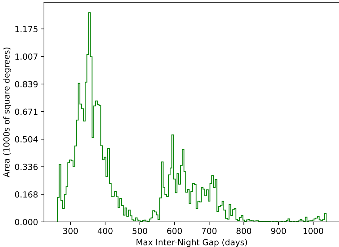
ddf_acor_sf20_lsf30_lsr10_v3.4_10yrs All sky g band: Max Inter-Night Gap
