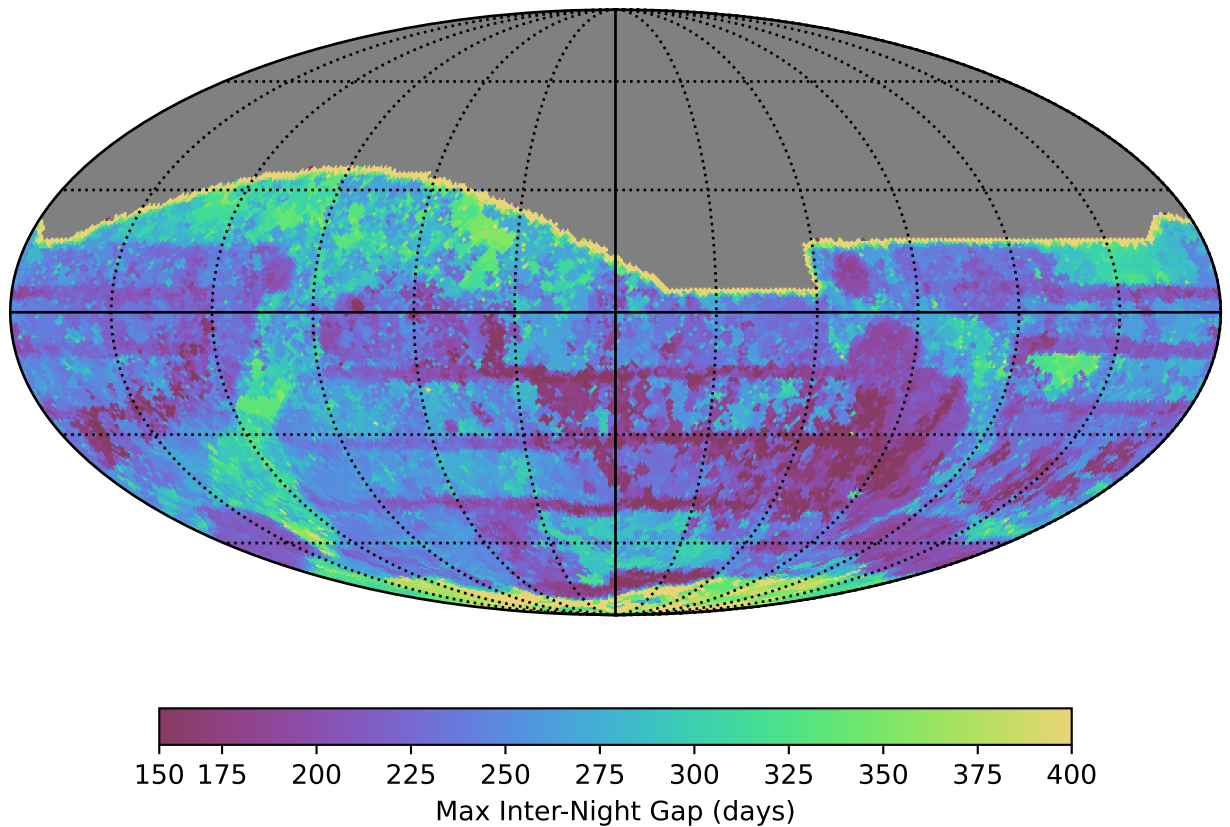
ddf_acor_sf20_lsf30_lsr10_v3.4_10yrs All sky all bands: Max Inter-Night Gap
