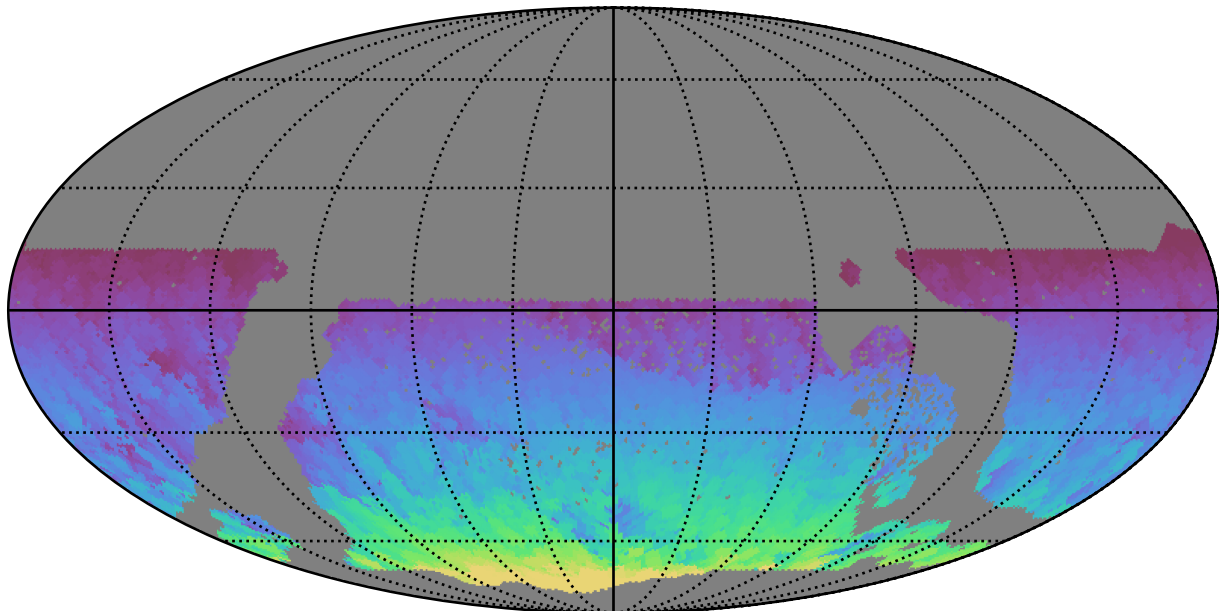
ddf_acor_sf20_lsf30_lsr10_v3.4_10yrs WFD all bands: Max HA
