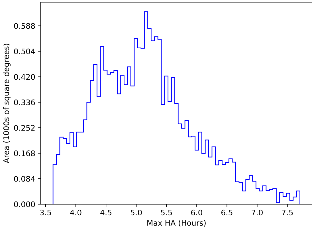
ddf_acor_sf20_lsf30_lsr10_v3.4_10yrs WFD all bands: Max HA
