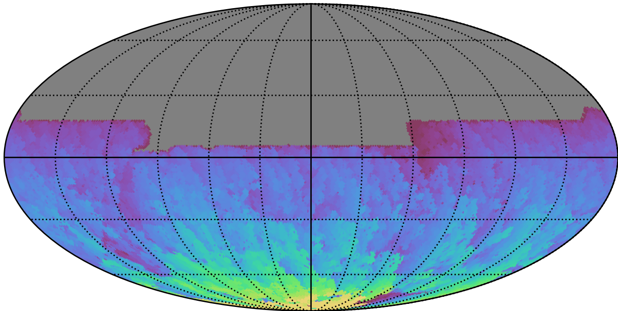
ddf_acor_sf20_lsf30_lsr10_v3.4_10yrs All sky y band: Max HA
