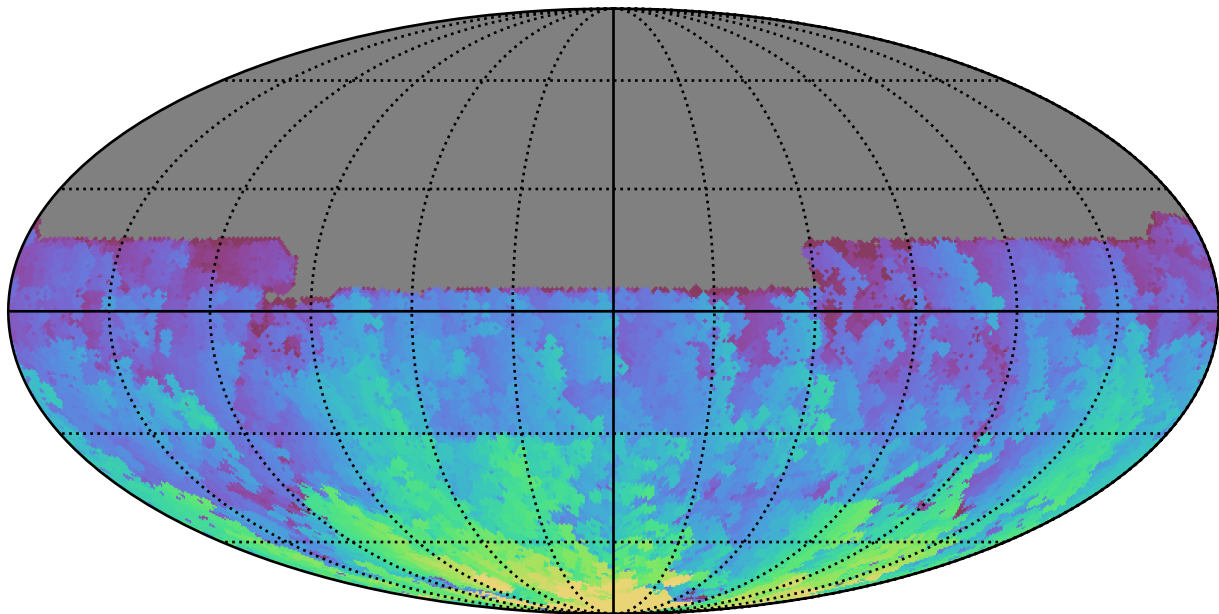
ddf_acor_sf20_lsf30_lsr10_v3.4_10yrs All sky u band: Max HA
