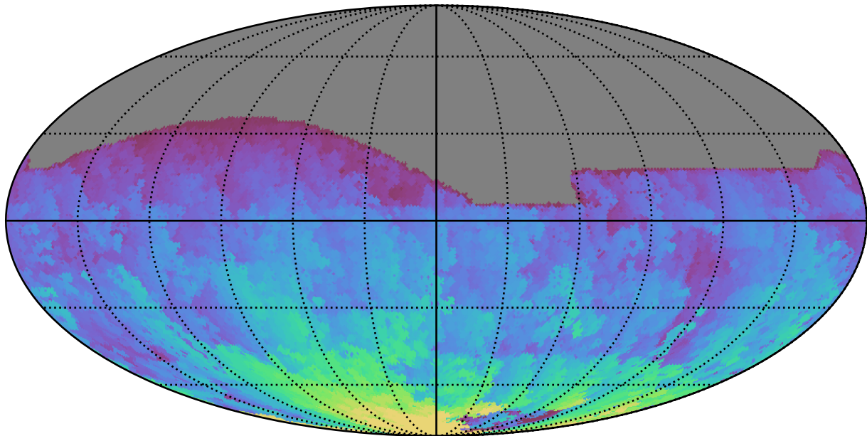
ddf_acor_sf20_lsf30_lsr10_v3.4_10yrs All sky r band: Max HA
