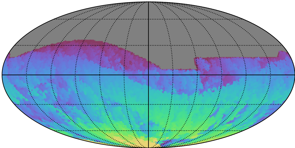
ddf_acor_sf20_lsf30_lsr10_v3.4_10yrs All sky i band: Max HA
