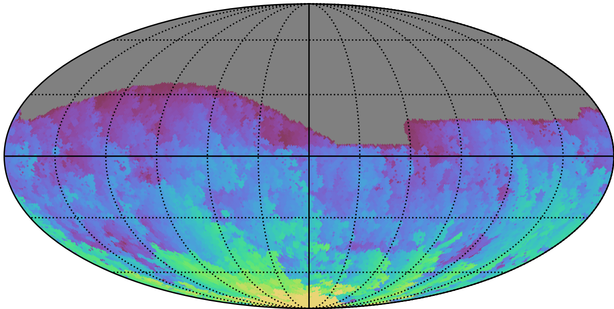
ddf_acor_sf20_lsf30_lsr10_v3.4_10yrs All sky g band: Max HA
