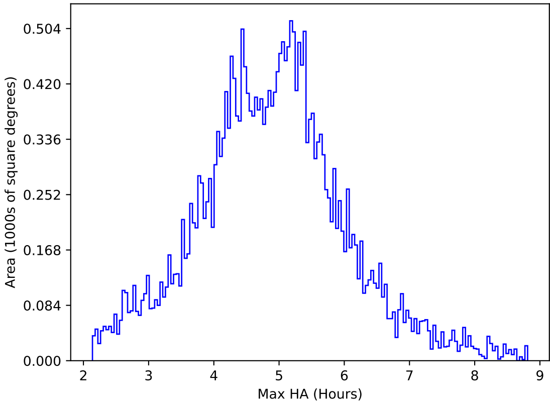
ddf_acor_sf20_lsf30_lsr10_v3.4_10yrs All sky all bands: Max HA
