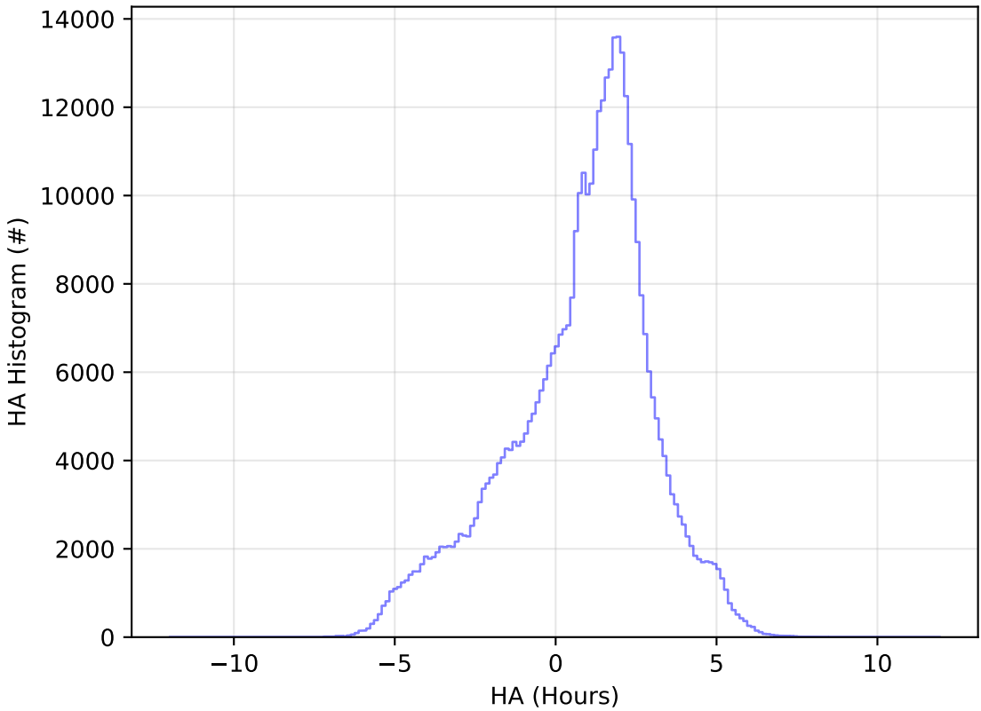
ddf_acor_sf20_lsf30_lsr10_v3.4_10yrs WFD z band: HA Histogram
