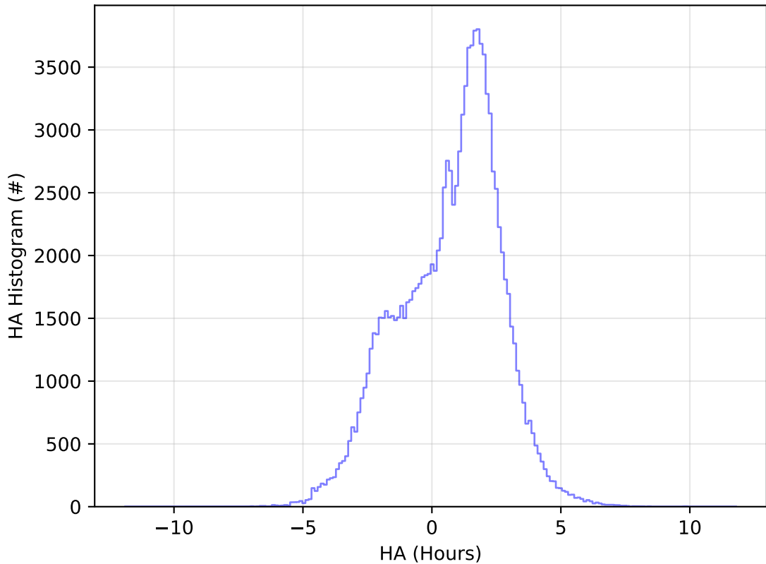
ddf_acor_sf20_lsf30_lsr10_v3.4_10yrs WFD u band: HA Histogram
