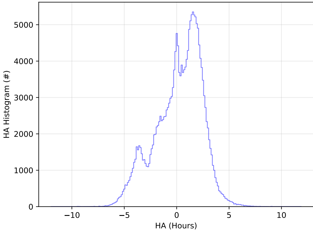
ddf_acor_sf20_lsf30_lsr10_v3.4_10yrs WFD g band: HA Histogram
