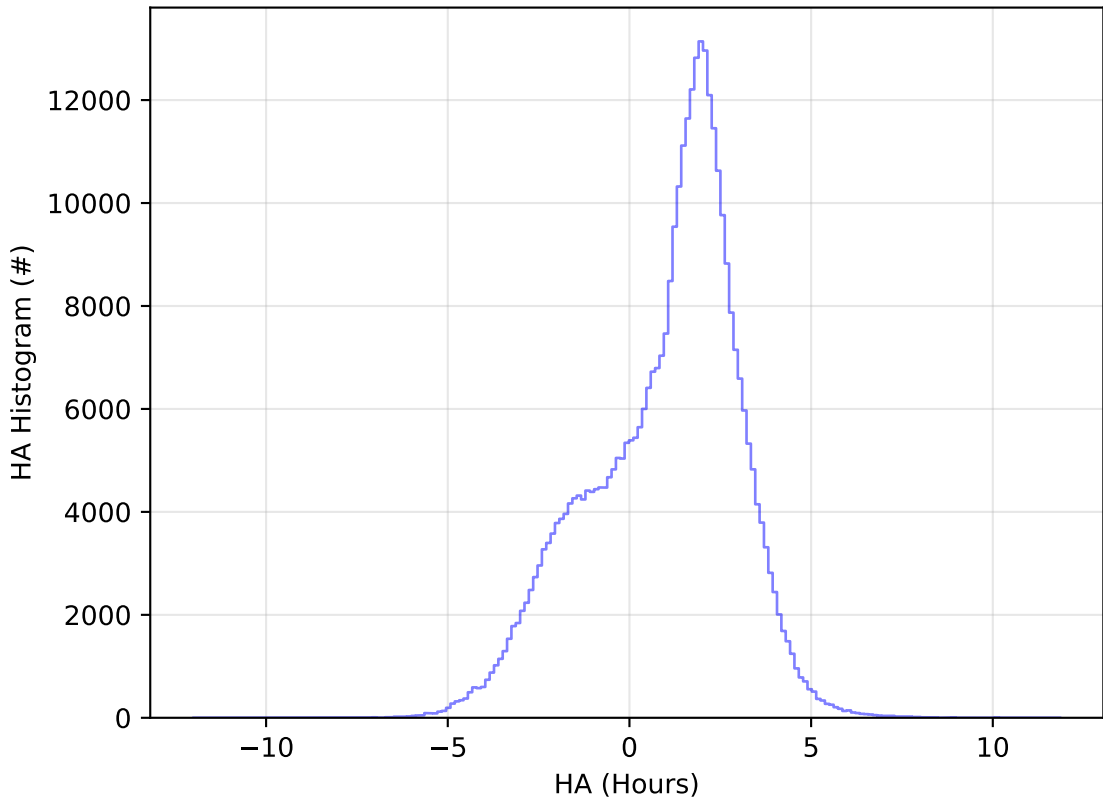
ddf_acor_sf20_lsf30_lsr10_v3.4_10yrs All sky y band: HA Histogram
