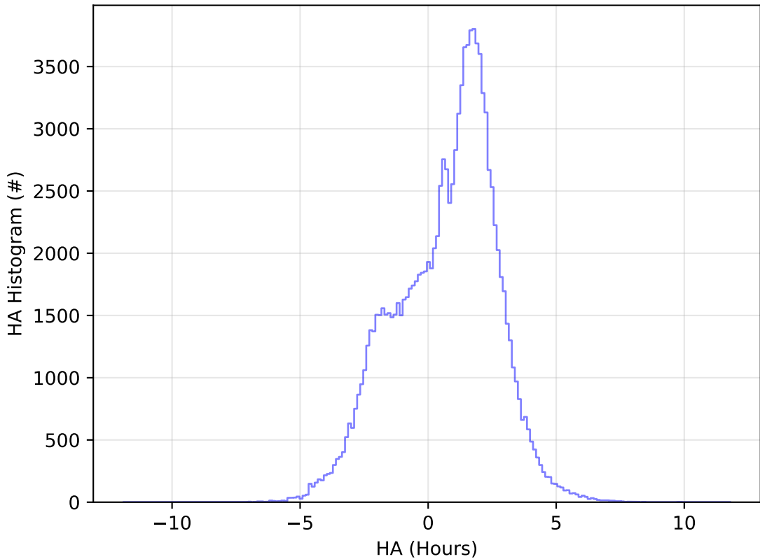
ddf_acor_sf20_lsf30_lsr10_v3.4_10yrs All sky u band: HA Histogram
