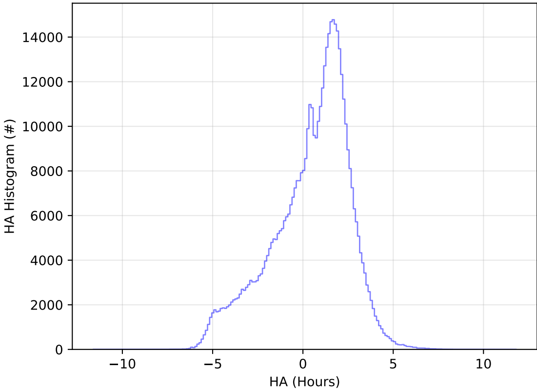
ddf_acor_sf20_lsf30_lsr10_v3.4_10yrs All sky r band: HA Histogram
