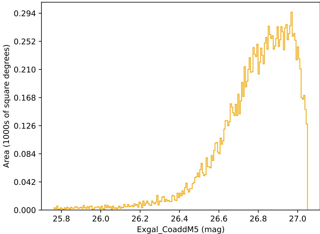
ddf_acor_sf20_lsf30_lsr10_v3.4_10yrs WFD r band: Exgal_CoaddM5
