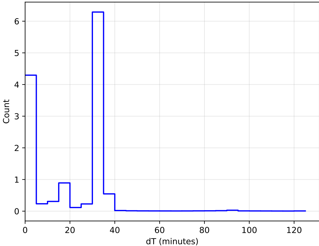
ddf_acor_sf20_lsf30_lsr10_v3.4_10yrs All sky: DeltaT Histogram
