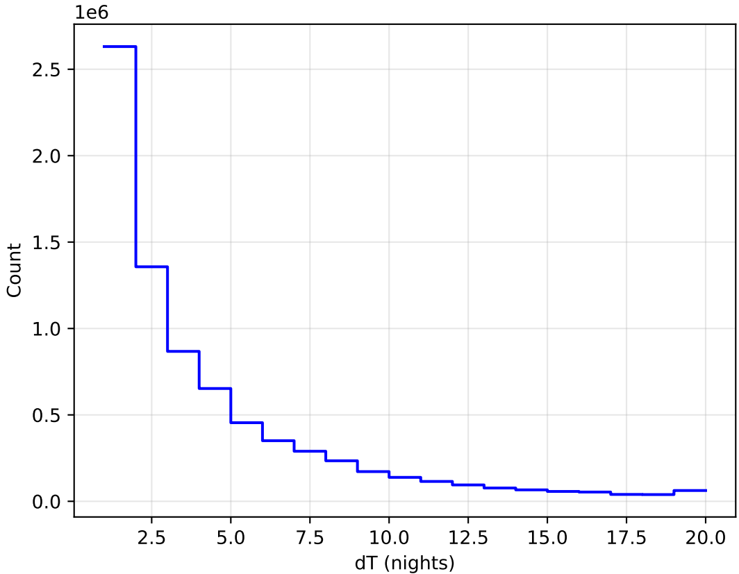
ddf_acor_sf20_lsf30_lsr10_v3.4_10yrs WFD all bands: DeltaNight Histogram
