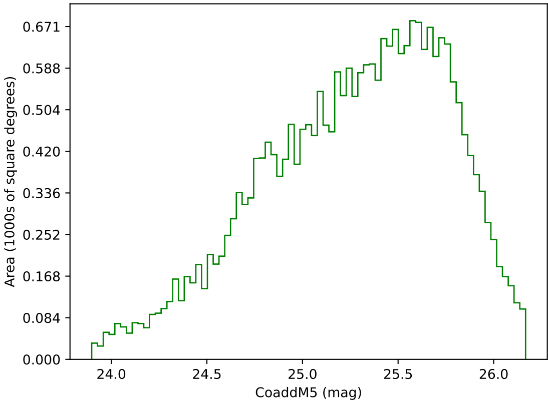
ddf_acor_sf20_lsf30_lsr10_v3.4_10yrs Yr 3-4 g band: CoaddM5
