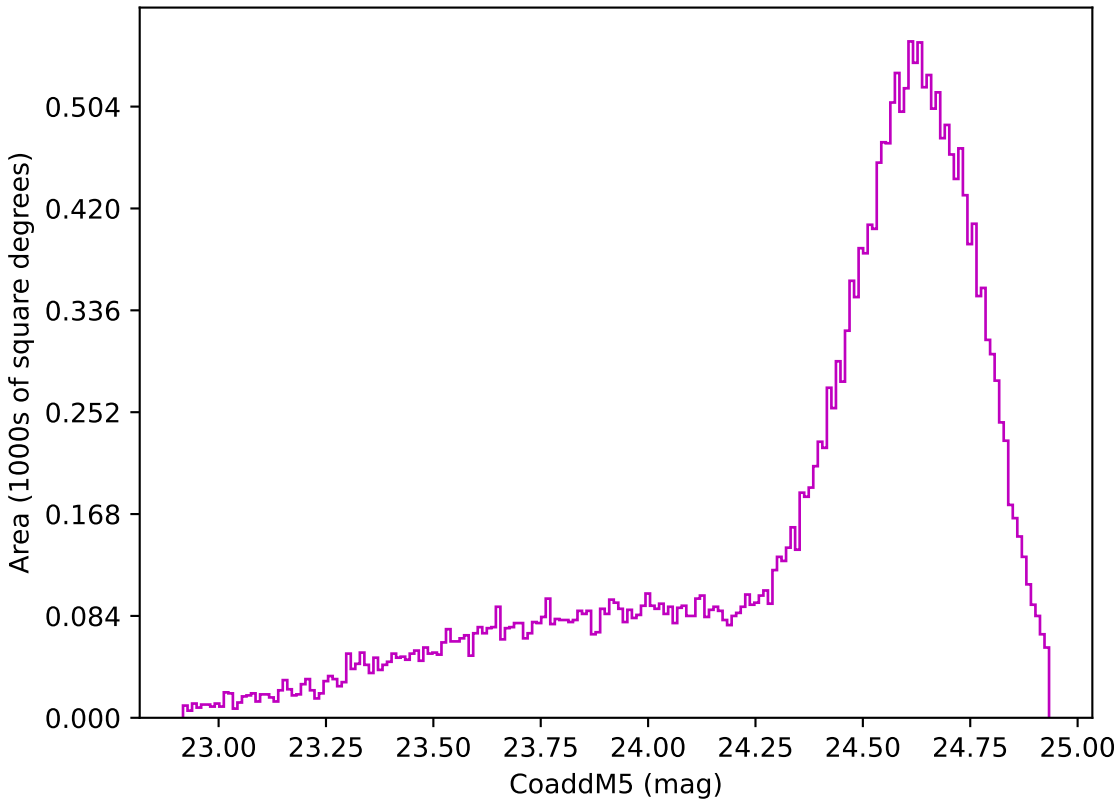
ddf_acor_sf20_lsf30_lsr10_v3.4_10yrs Yr 1 z band: CoaddM5
