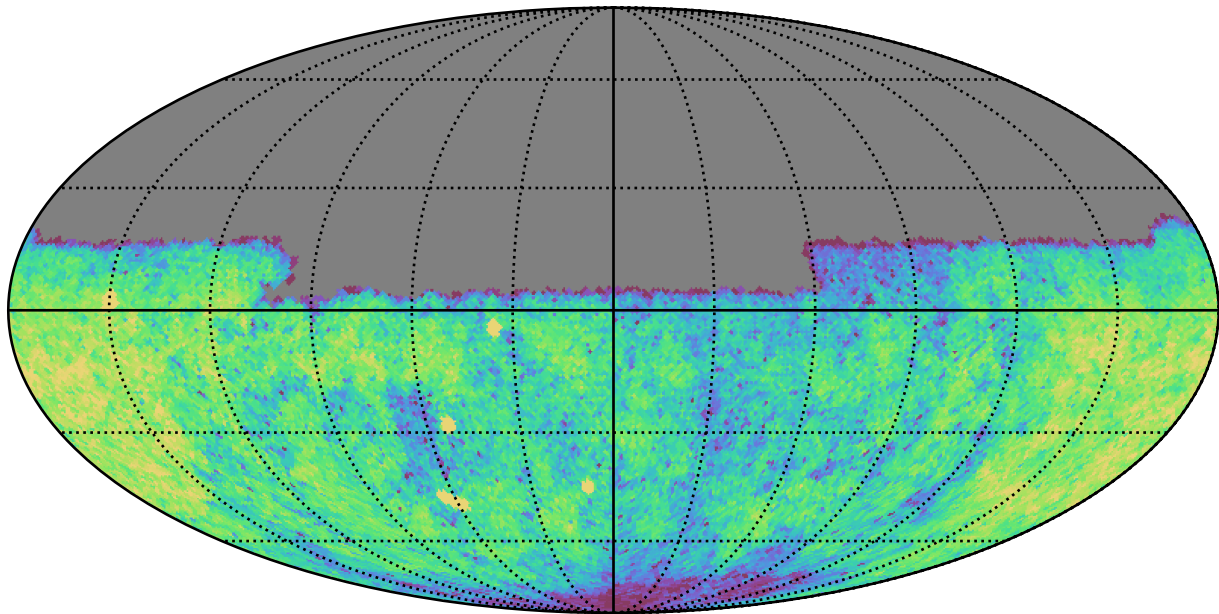
ddf_acor_sf20_lsf30_lsr10_v3.4_10yrs Yr 1 u band: CoaddM5
