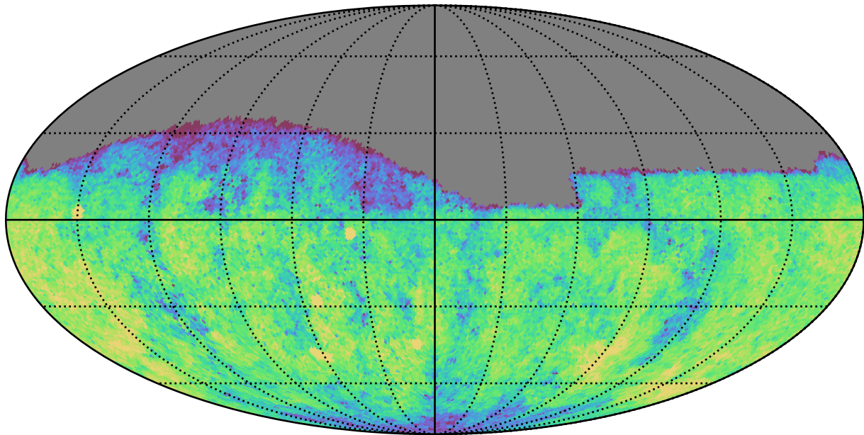
ddf_acor_sf20_lsf30_lsr10_v3.4_10yrs Yr 1 g band: CoaddM5
