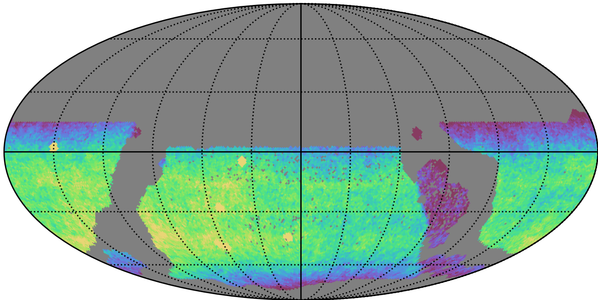
ddf_acor_sf20_lsf30_lsr10_v3.4_10yrs WFD y band: CoaddM5
