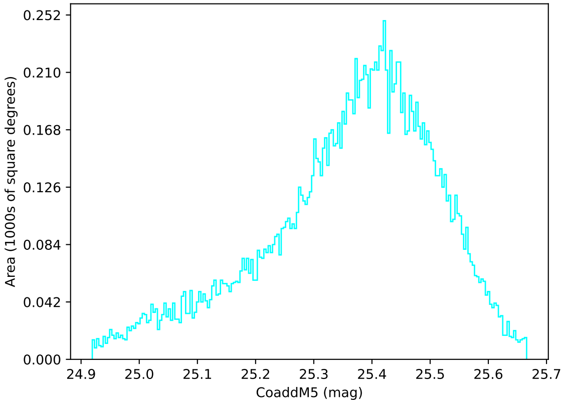
ddf_acor_sf20_lsf30_lsr10_v3.4_10yrs WFD u band: CoaddM5
