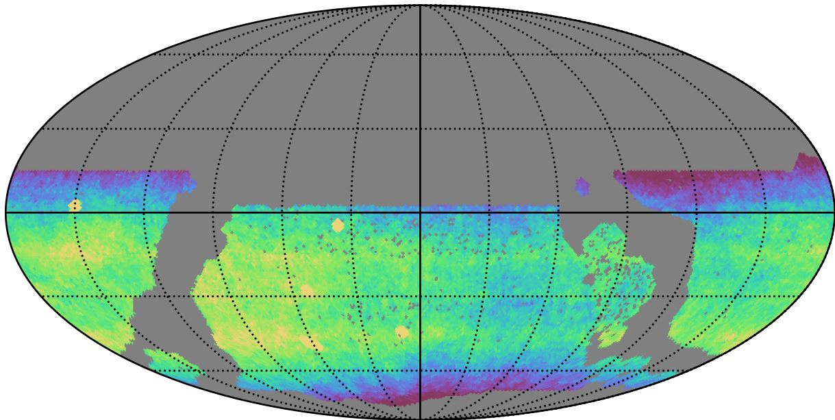
ddf_acor_sf20_lsf30_lsr10_v3.4_10yrs WFD i band: CoaddM5
