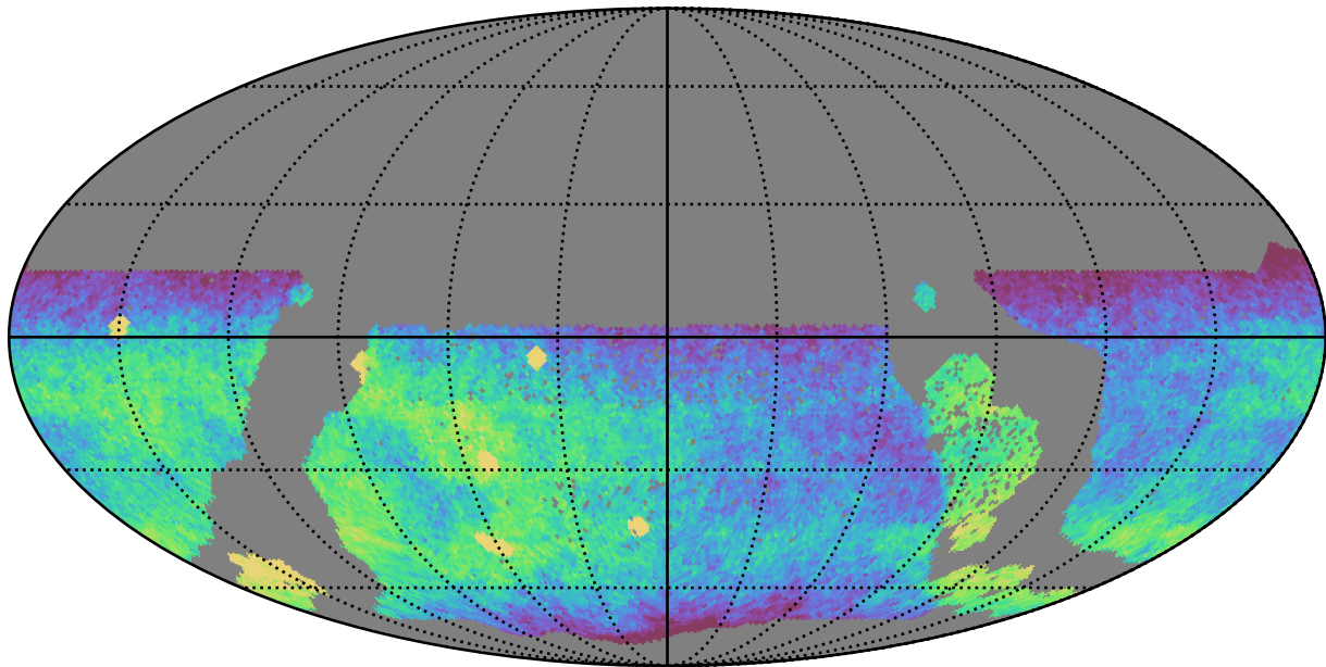
ddf_acor_sf20_lsf30_lsr10_v3.4_10yrs WFD g band: CoaddM5
