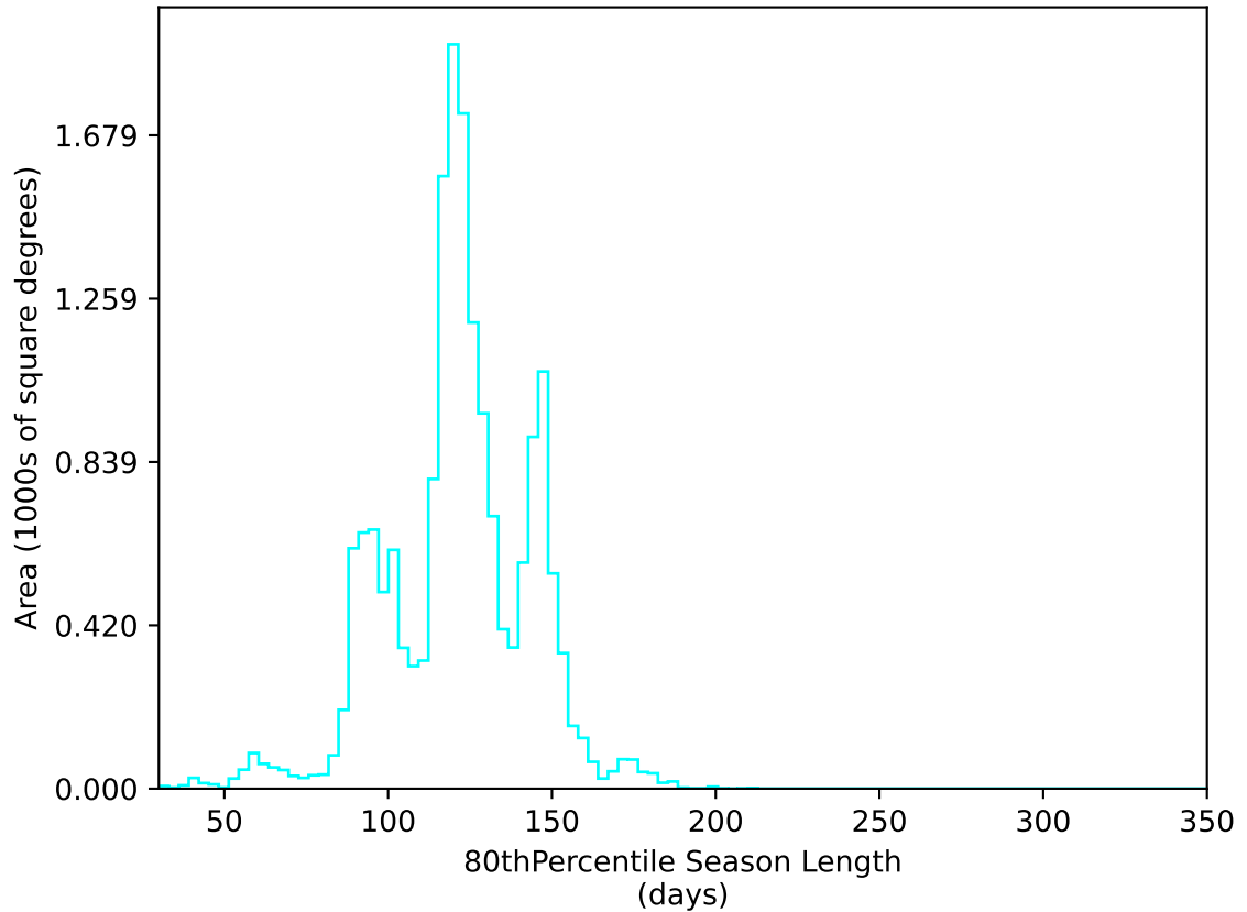
ddf_acor_sf20_ls30_lsr10_v3.4_10yrs WFD u band: 80thPercentile Season Length
