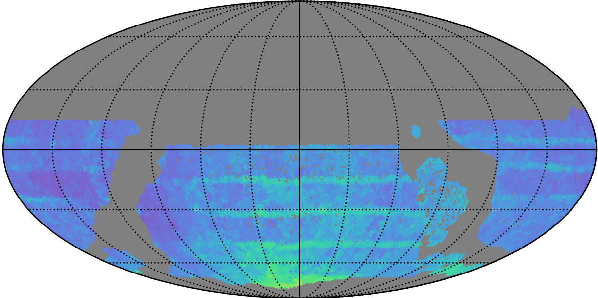
ddf_acor_sf20_lsf30_lsr10_v3.4_10yrs WFD all bands: 80thPercentile Season Length
