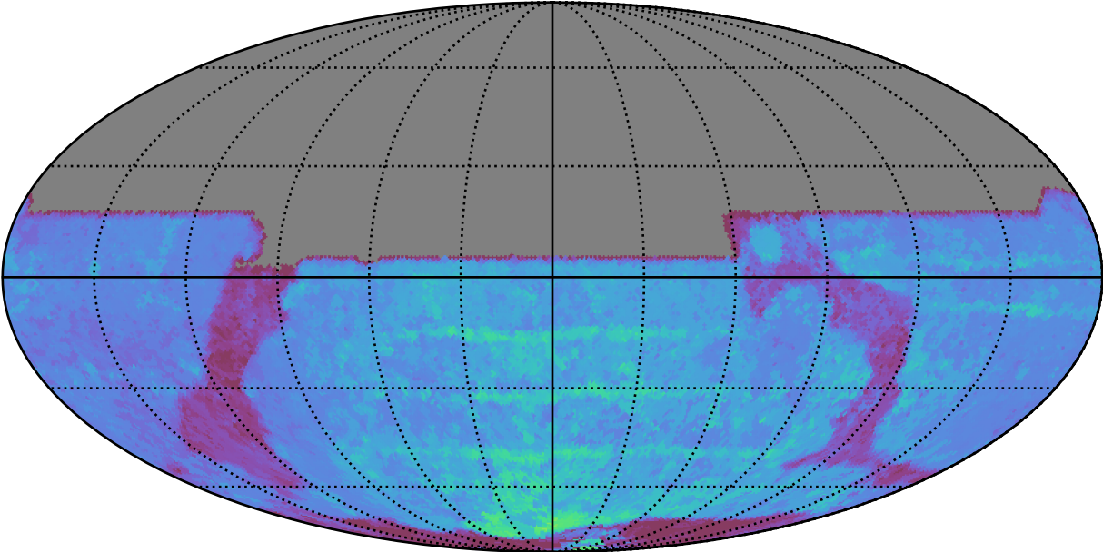
ddf_acor_sf20_lsf30_lsr10_v3.4_10yrs All sky y band: 80thPercentile Season Length
