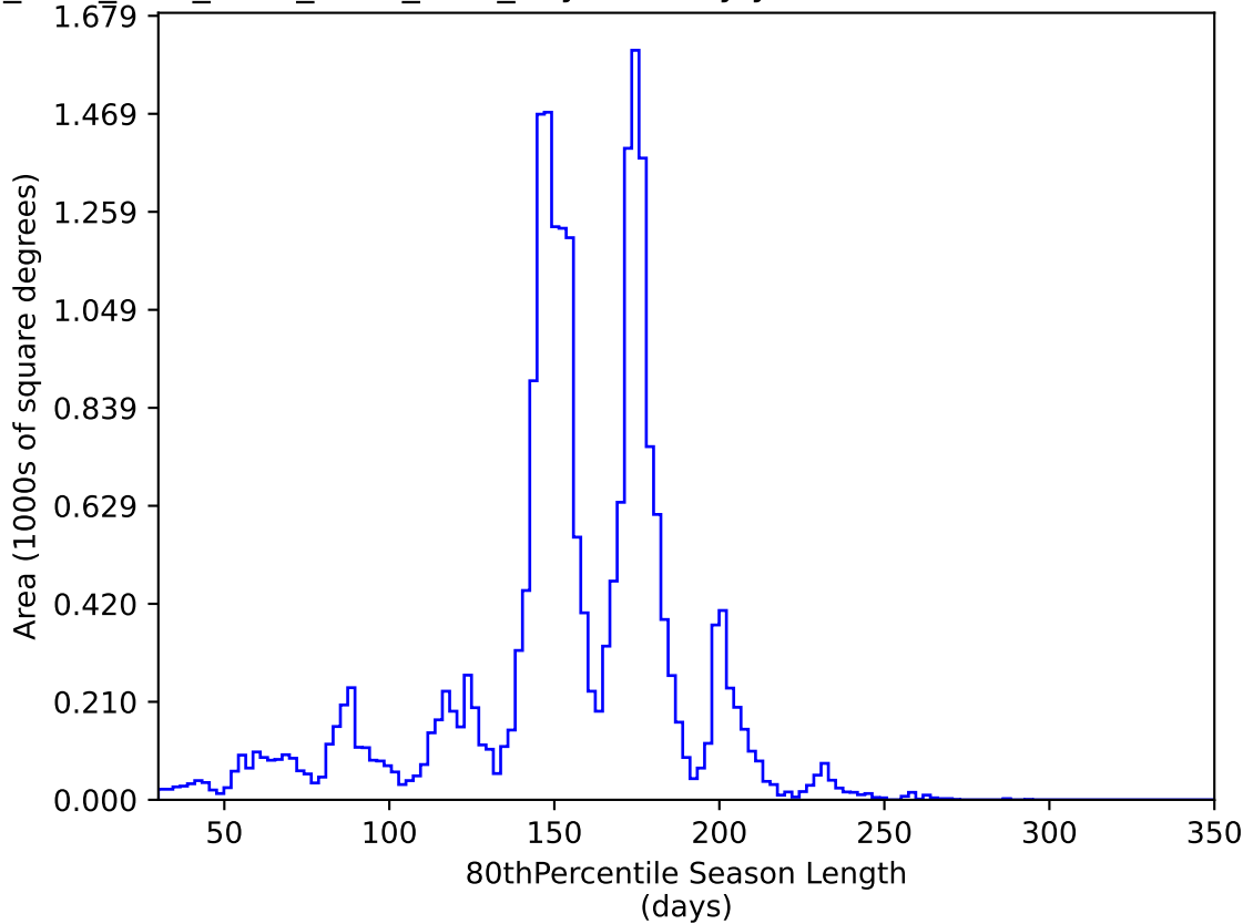
ddf_acor_sf20_lsf30_lsr10_v3.4_10yrs All sky y band: 80thPercentile Season Length
