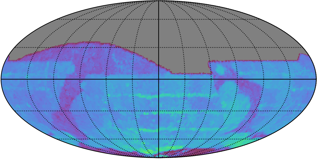
ddf_acor_sf20_lsf30_lsr10_v3.4_10yrs All sky r band: 80thPercentile Season Length
