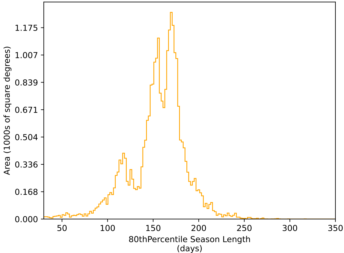
ddf_acor_sf20_lsf30_lsr10_v3.4_10yrs All sky r band: 80thPercentile Season Length
