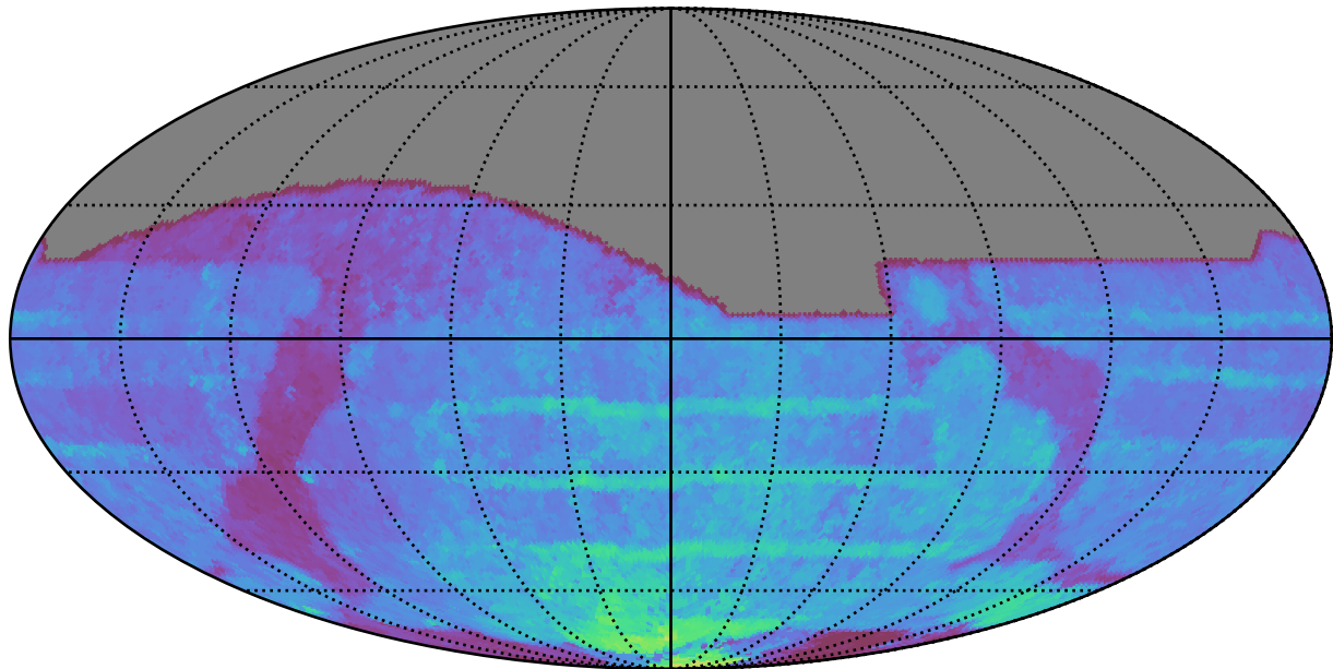
ddf_acor_sf20_lsf30_lsr10_v3.4_10yrs All sky all bands: 80thPercentile Season Length
