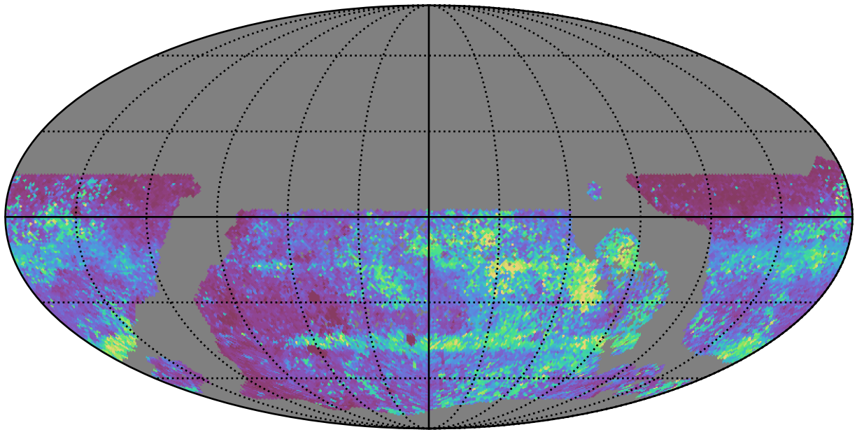
ddf_acor_sf20_lsf30_lsr10_v3.4_10yrs WFD zy bands: 75th Percentile Intranight Timespan
