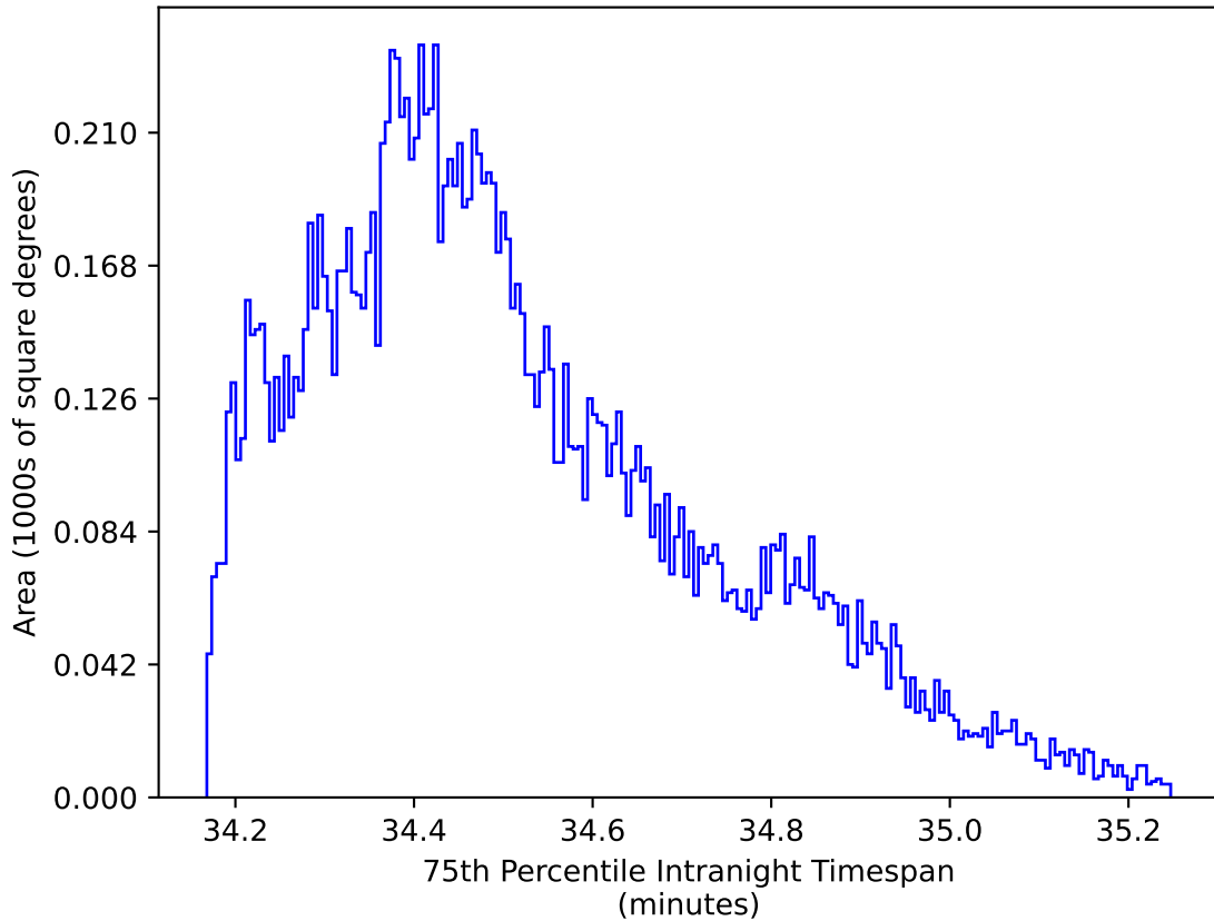
ddf_acor_sf20_lsf30_lsr10_v3.4_10yrs WFD zy bands: 75th Percentile Intranight Timespan
