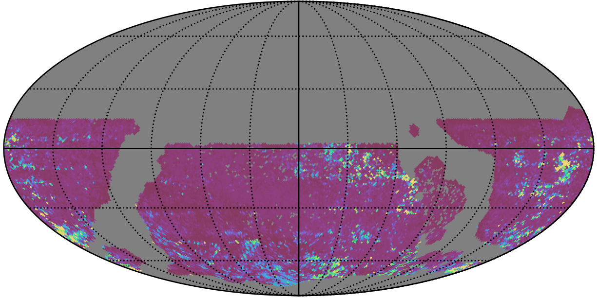
ddf_acor_sf20_lsf30_lsr10_v3.4_10yrs WFD z band: 75th Percentile Intranight Timespan
