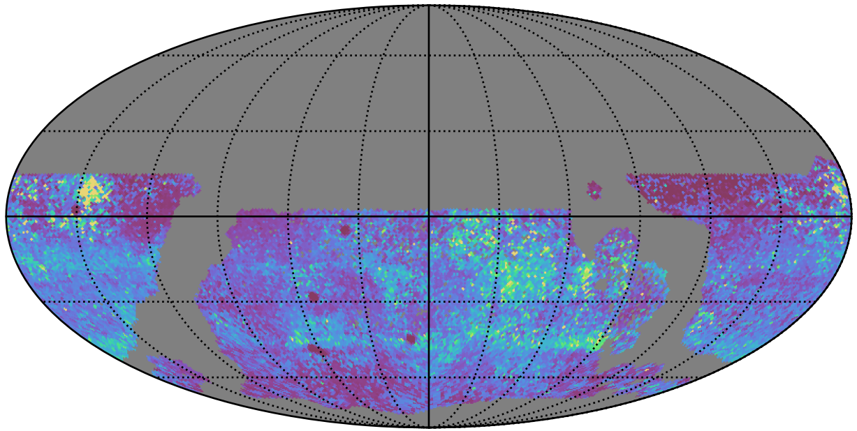
ddf_acor_sf20_lsr30_lsr10_v3.4_10yrs WFD y band: 75th Percentile Intranight Timespan
