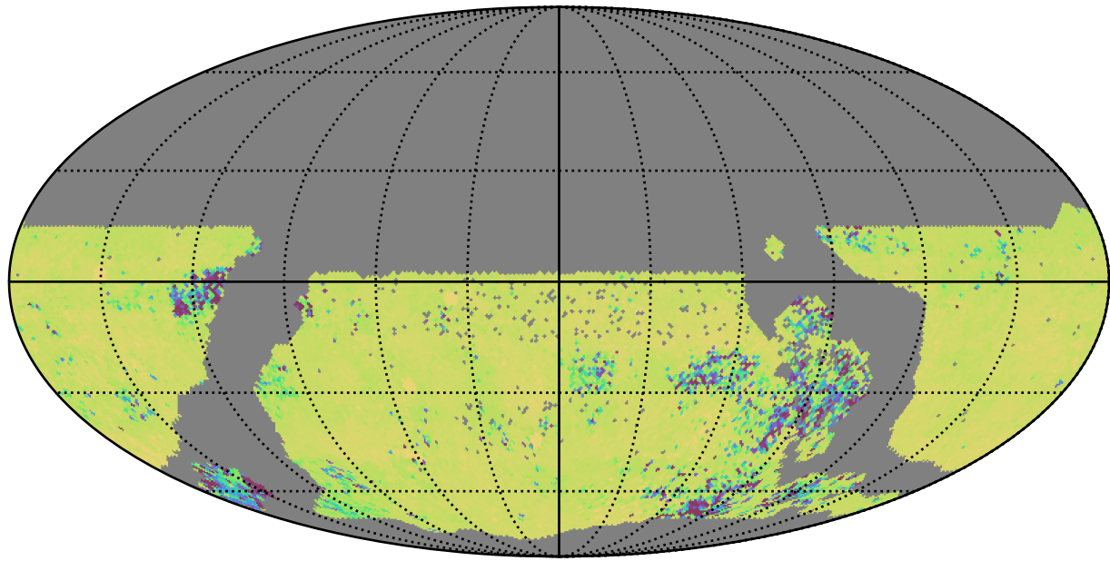
ddf_acor_sf20_lsf30_lsr10_v3.4_10yrs WFD ug bands: 75th Percentile Intranight Timespan
